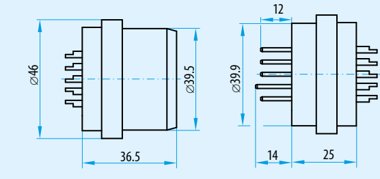
Dimensions insulator (socket piece/pin piece)
