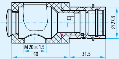
Socket piece
