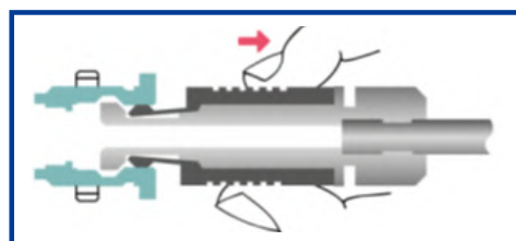
Pull the Outer Sleeve to Unlock
