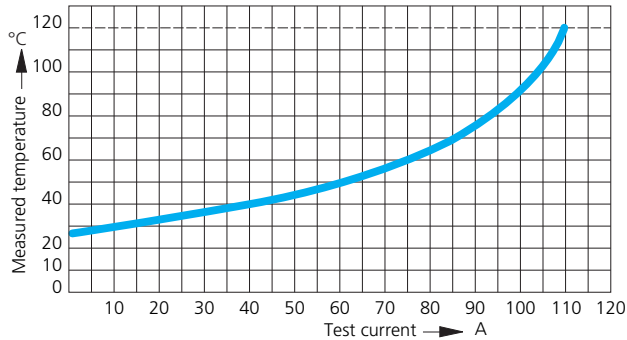
Springtac™ Socket Type 170-... Solid pin Type 180-... Contact Material Brass, silver-plated Contact-Ø 5 mm 16 mm² Cable Cross Section
