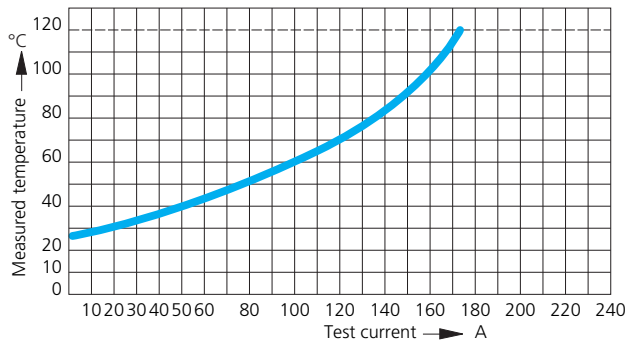
Springtac™ Socket Type 170-... Solid pin Type 180-... Contact Material Brass, silver-plated Contact-Ø 7 mm 35 mm² Cable Cross Section
