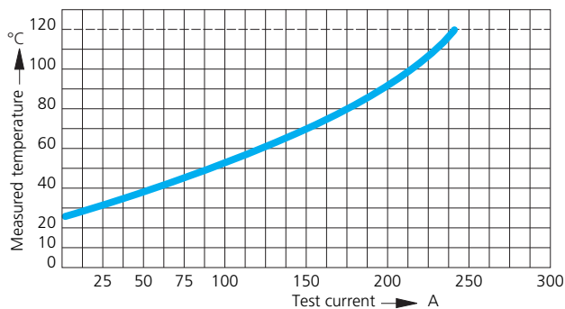
Springtac™ Socket Type 170-... Solid pin Type 180-... Contact Material Brass, silver-plated Contact-Ø 9 mm 50 mm² Cable Cross Section
