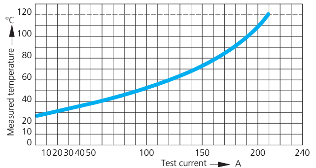
Springtac™ Socket Type 170-... Solid pin Type 180-... Contact Material Brass, silver-plated Contact-Ø 8 mm 50 mm² Cable Cross Section
